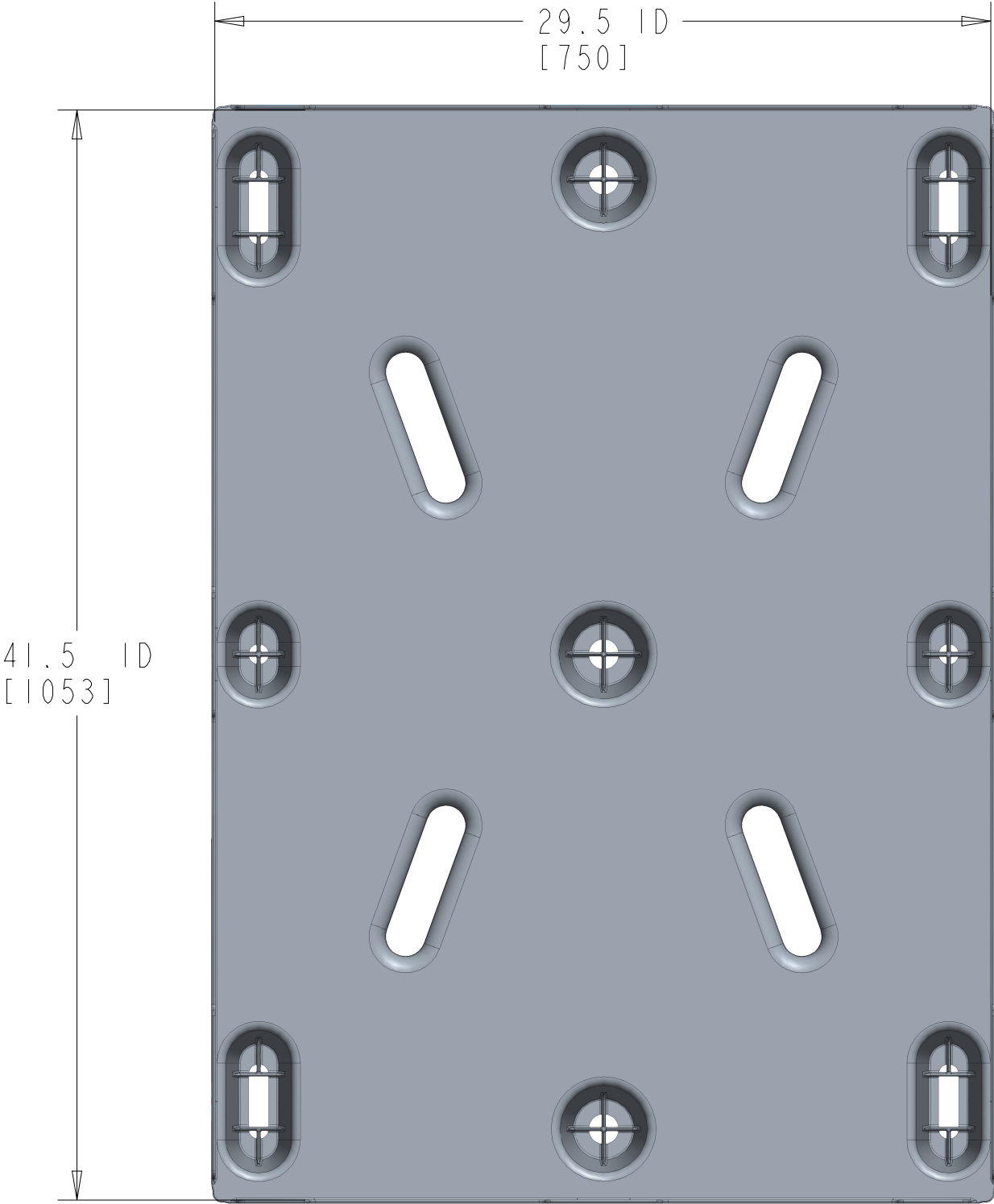
TOP VIEW
