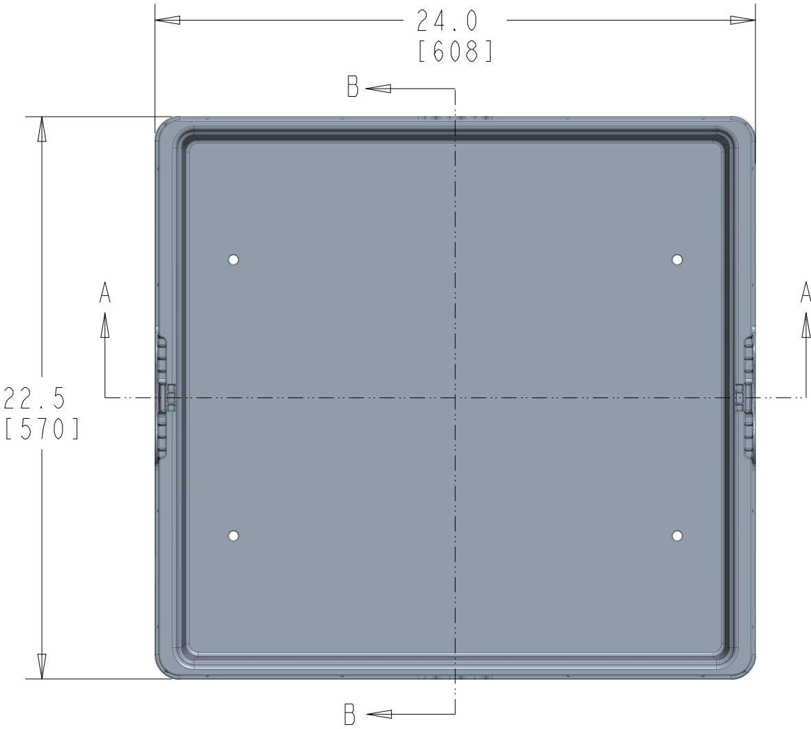
TOP VIEW
