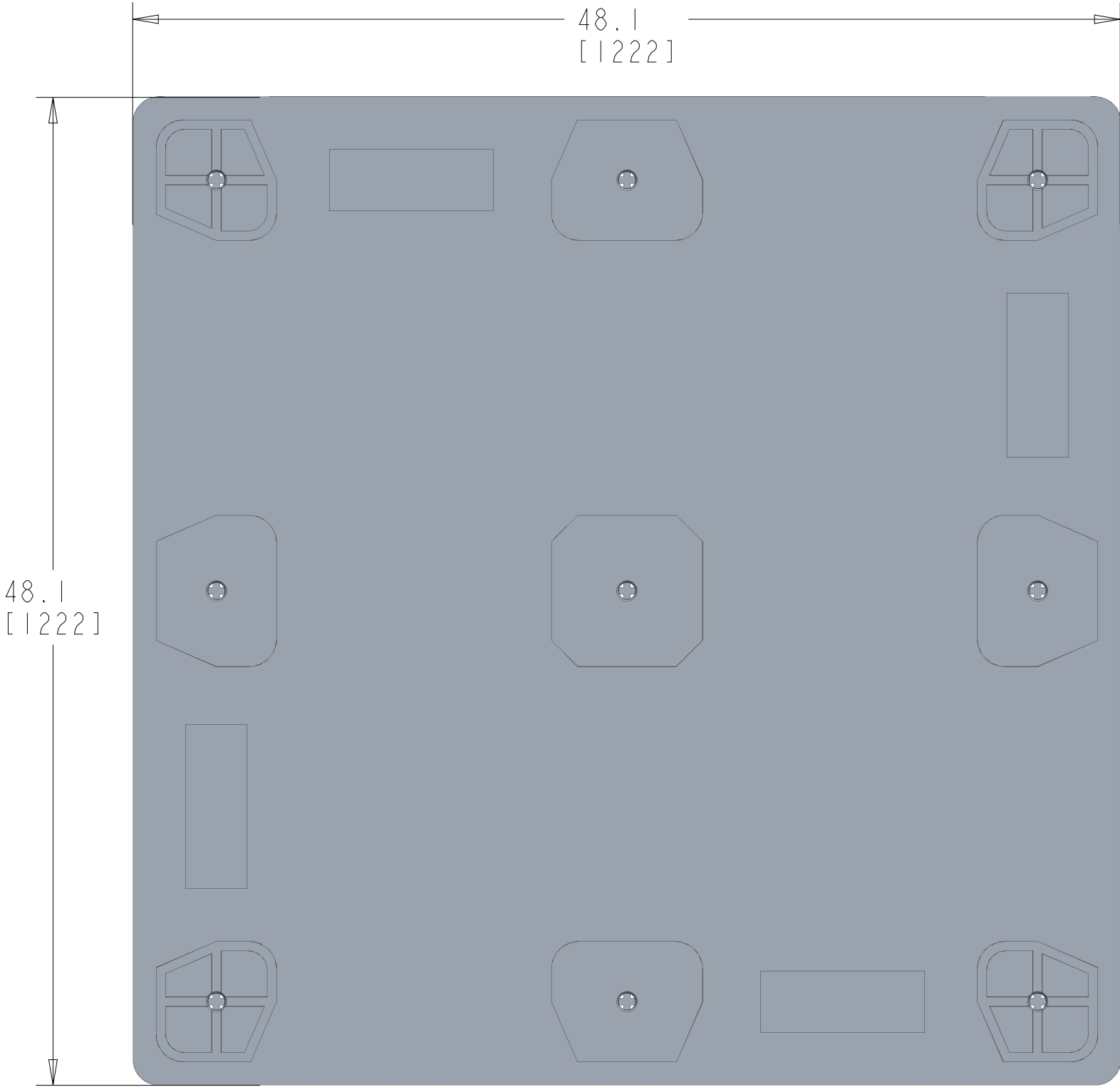
TOP VIEW
