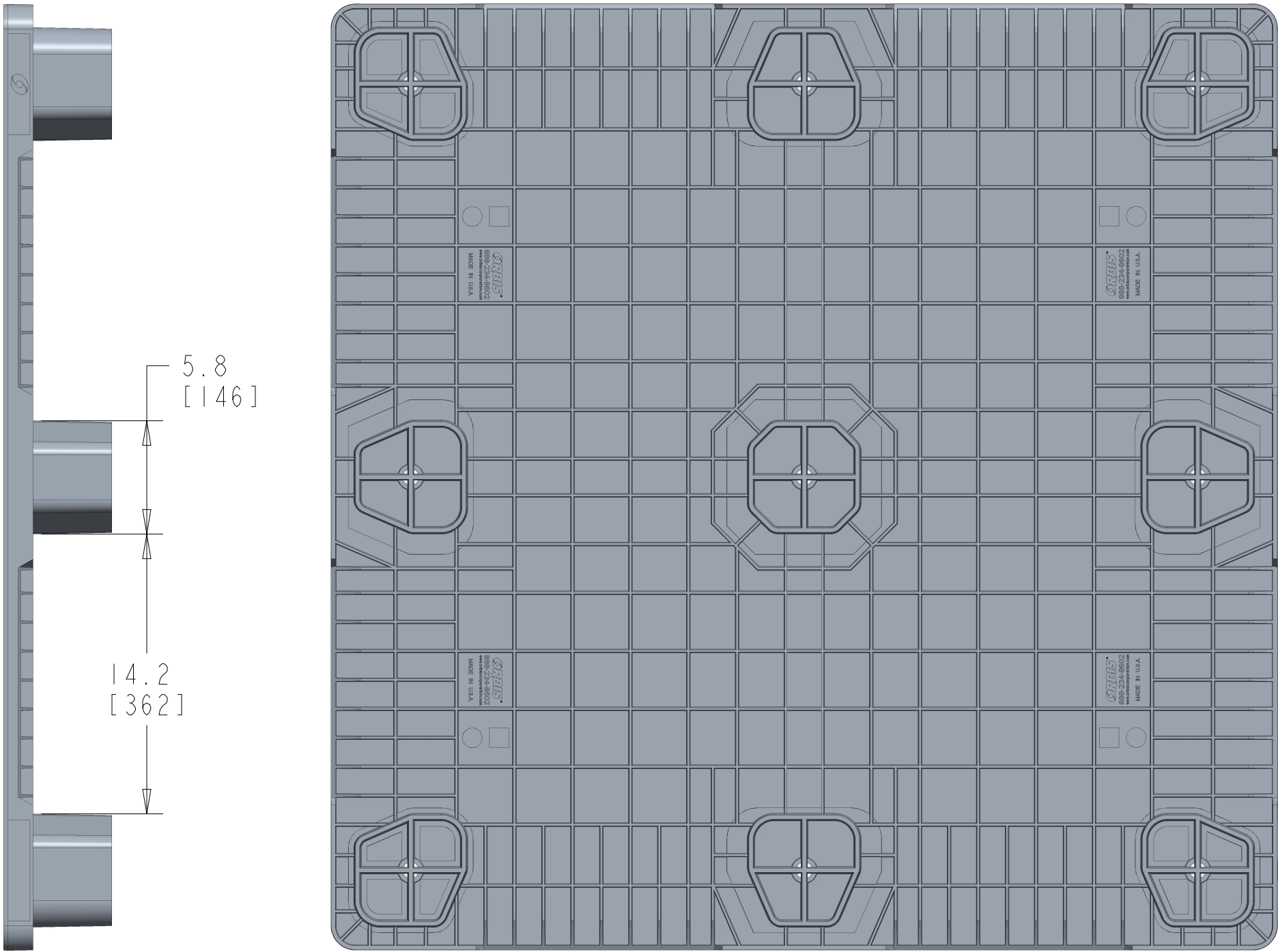
BOTTOM VIEW
