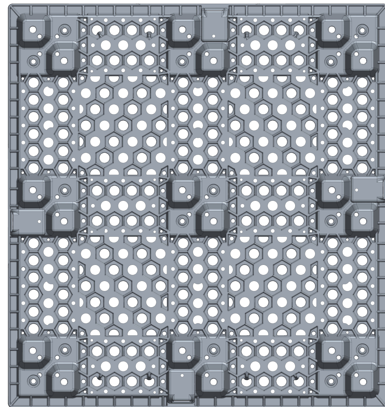
BOTTOM VIEW
