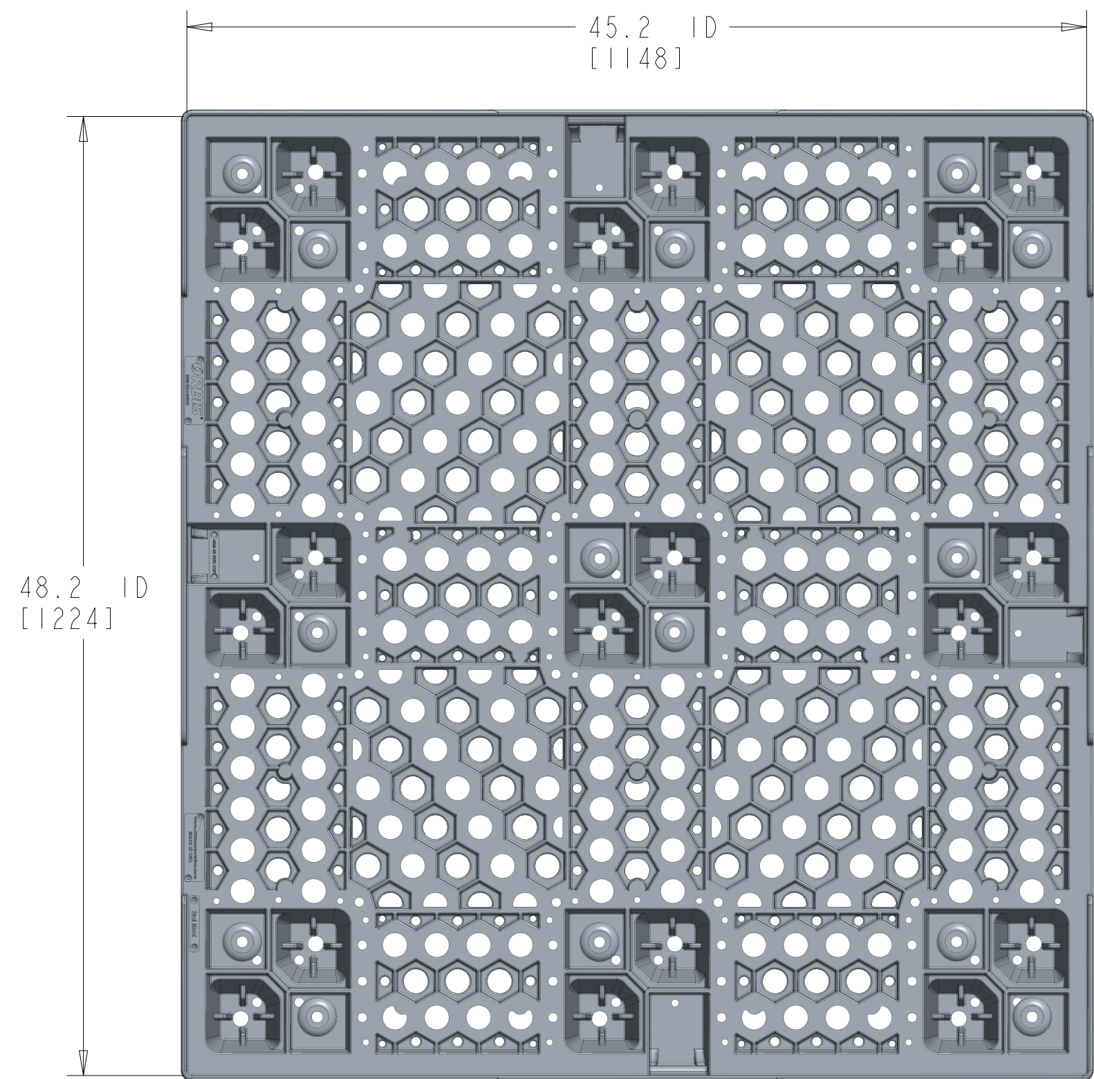
TOP VIEW
