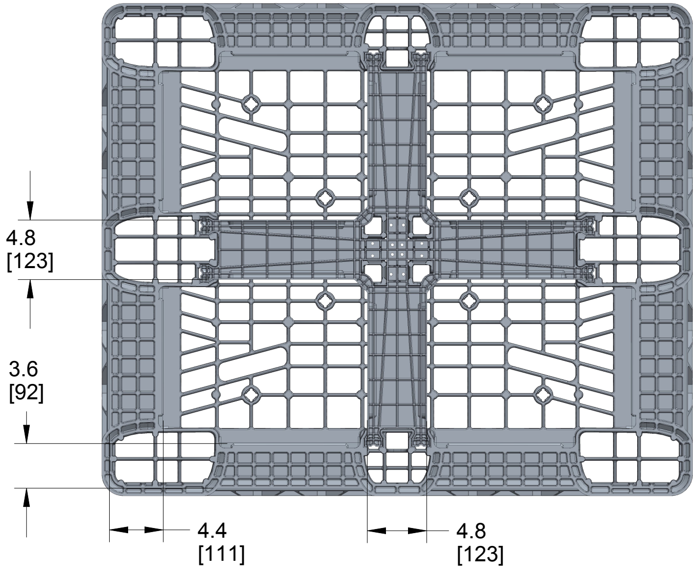
BOTTOM VIEW
