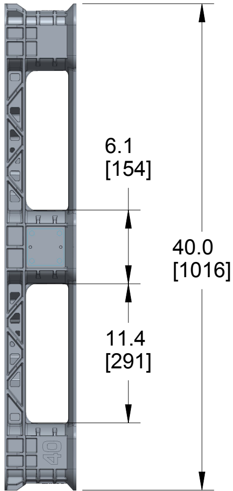
END VIEW
