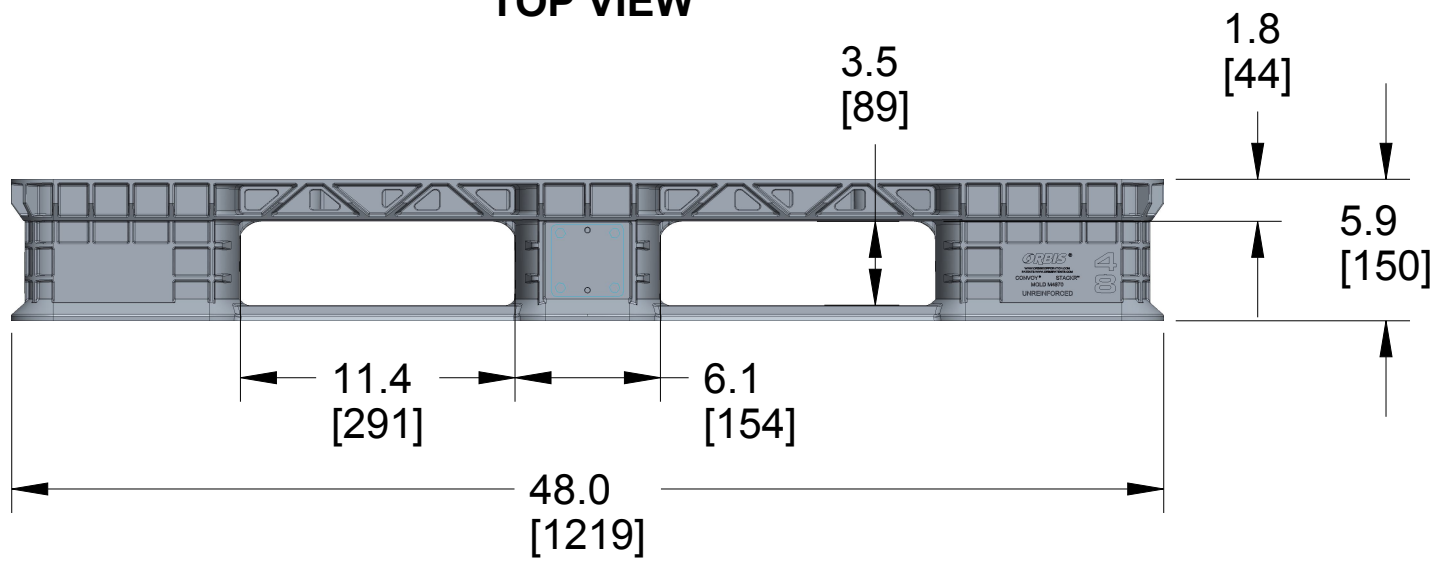
SIDE VIEW
