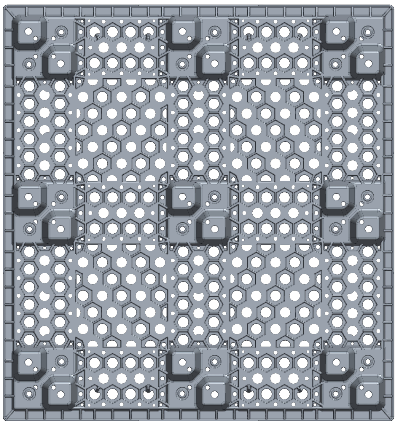
BOTTOM VIEW
