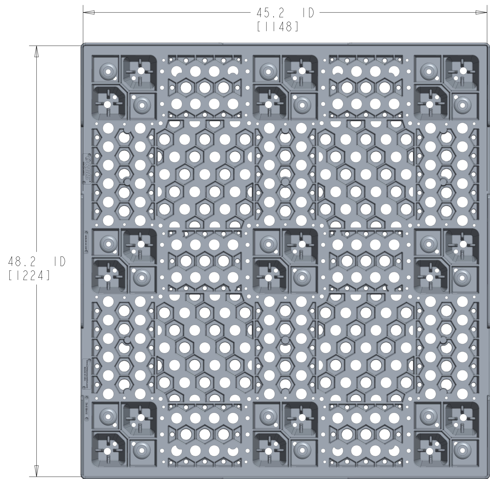
TOP VIEW
