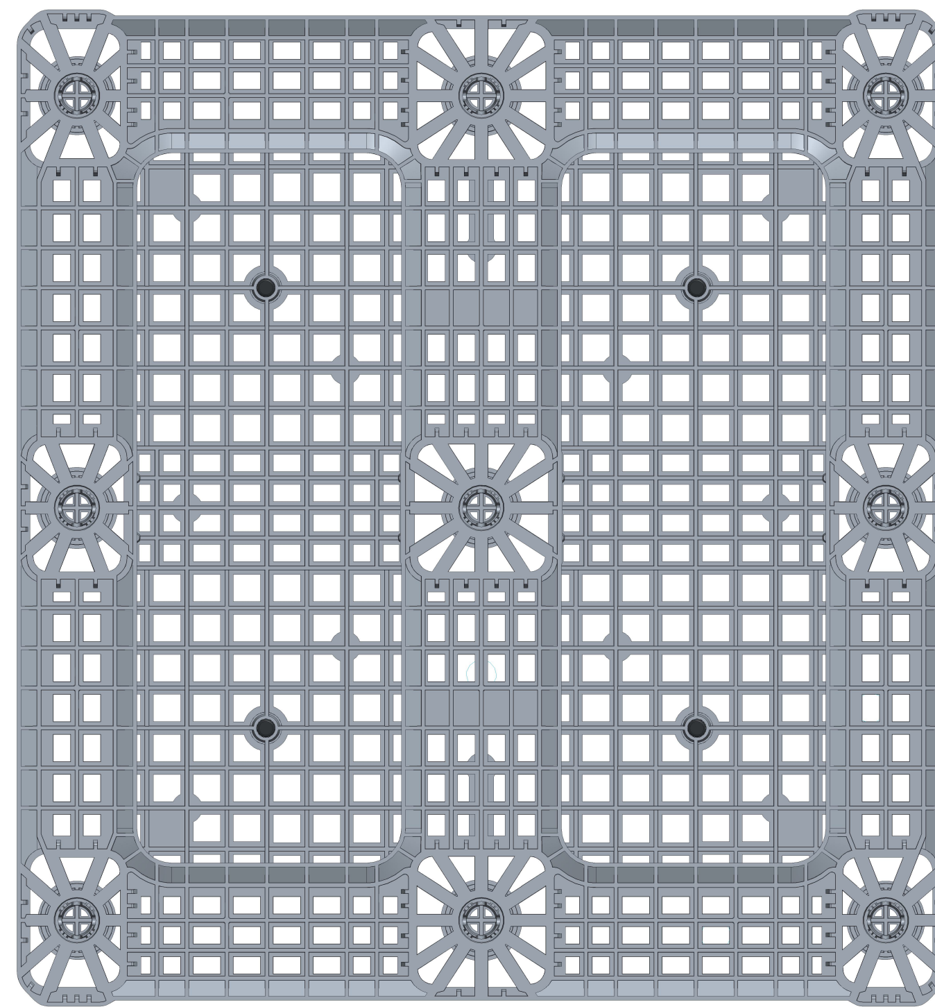
BOTTOM VIEW
