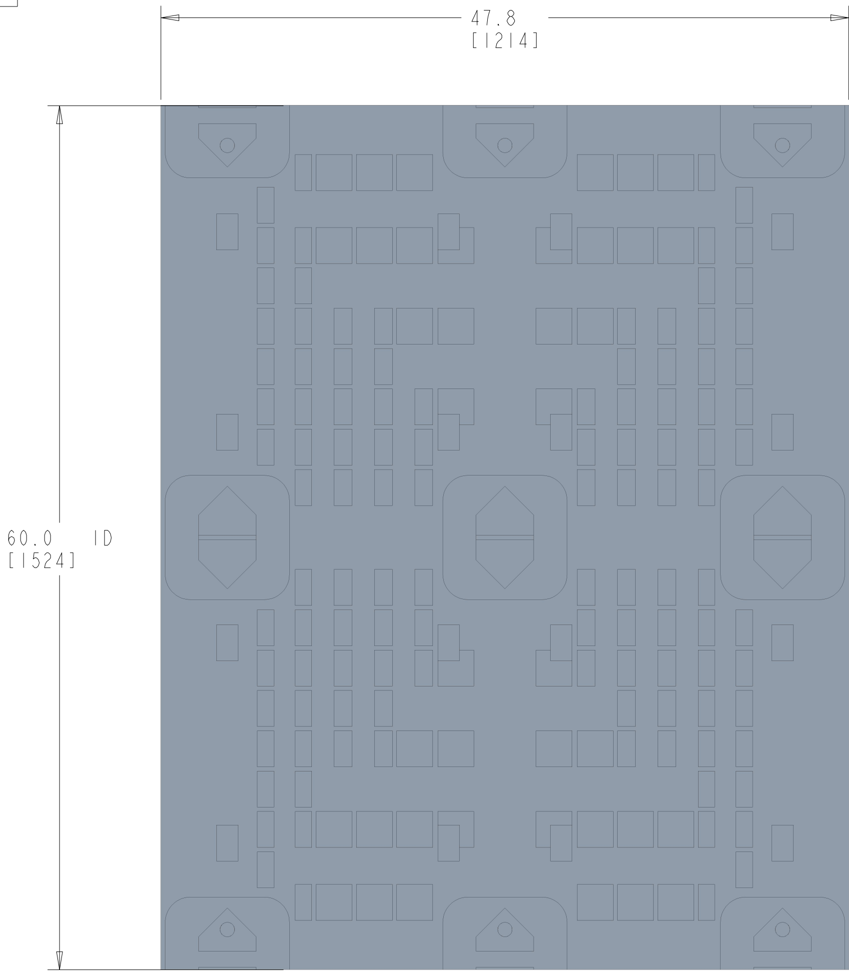
TOP VIEW
