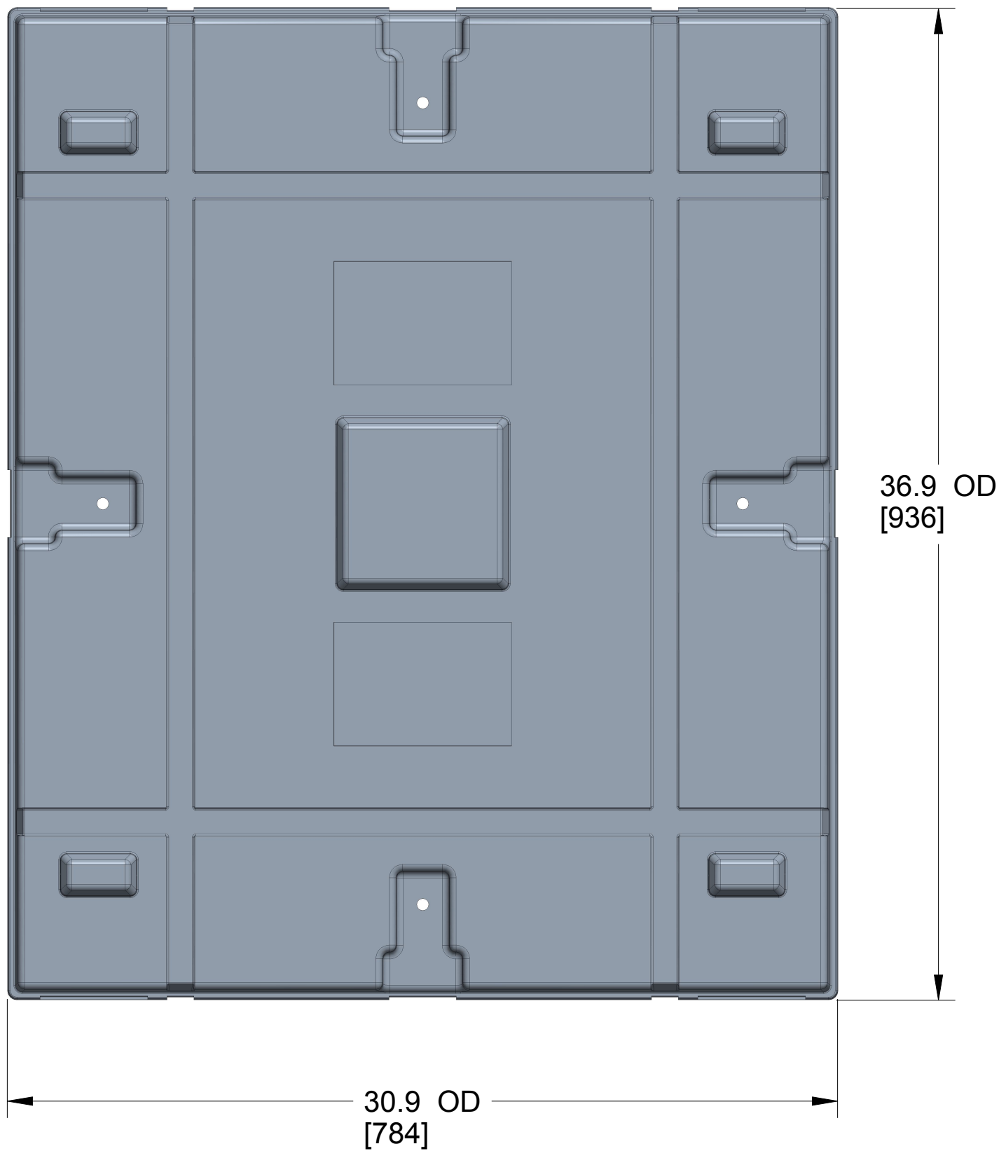
TOP VIEW
