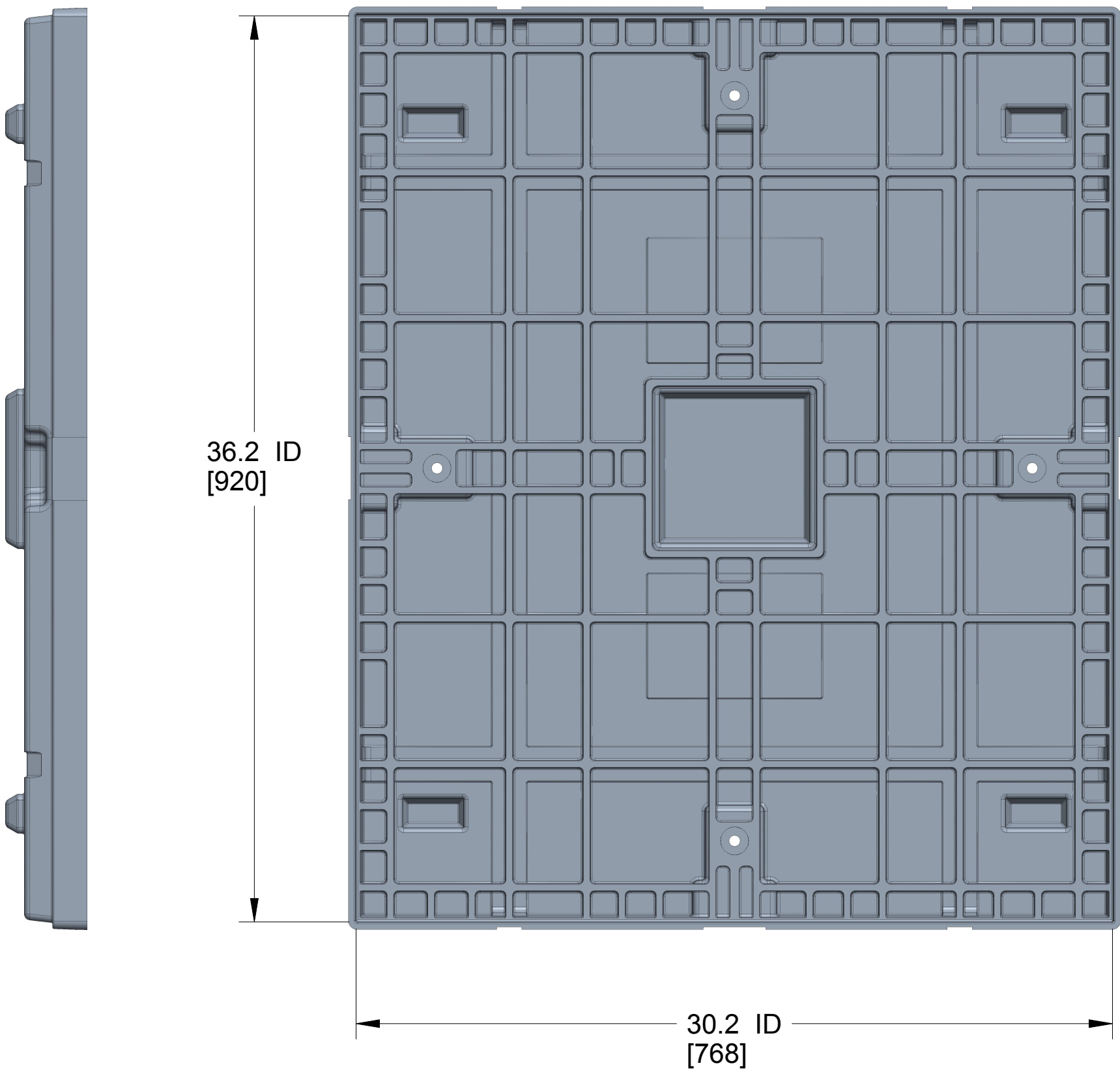
BOTTOM VIEW
