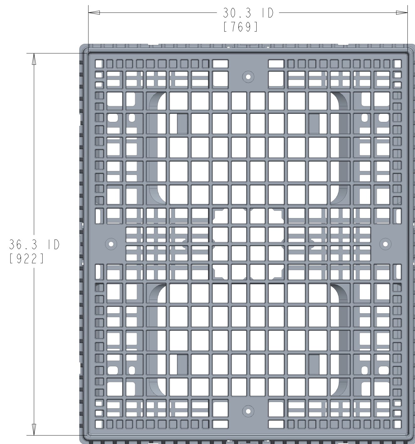
TOP VIEW
