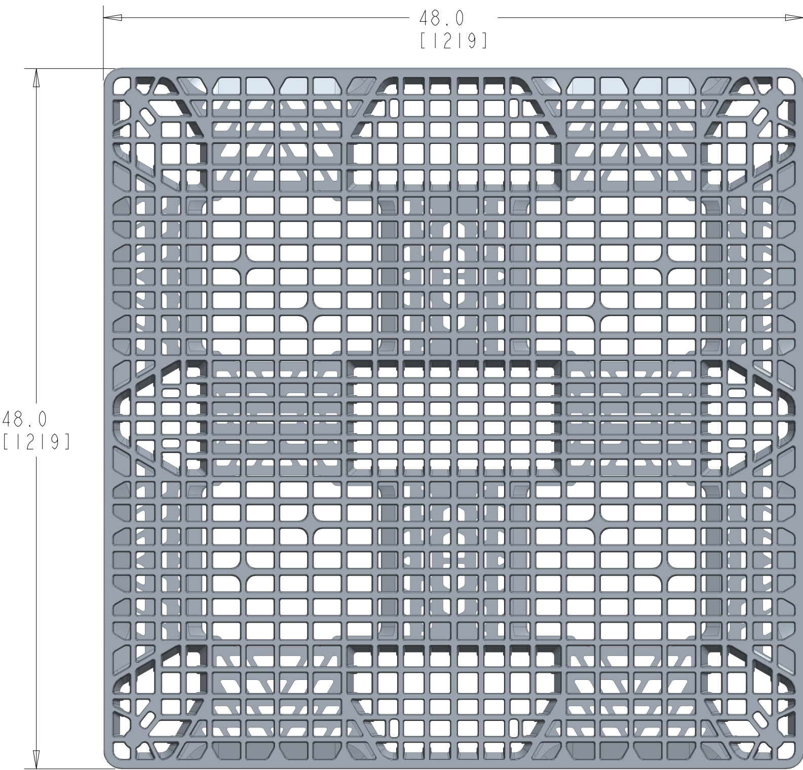
TOP VIEW
