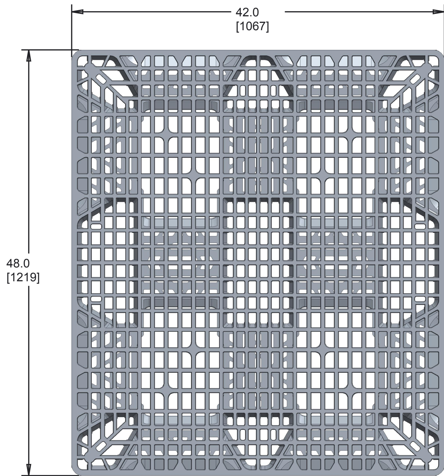
TOP VIEW
