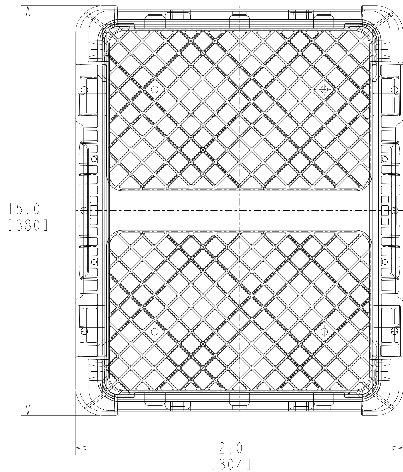
TOP VIEW
