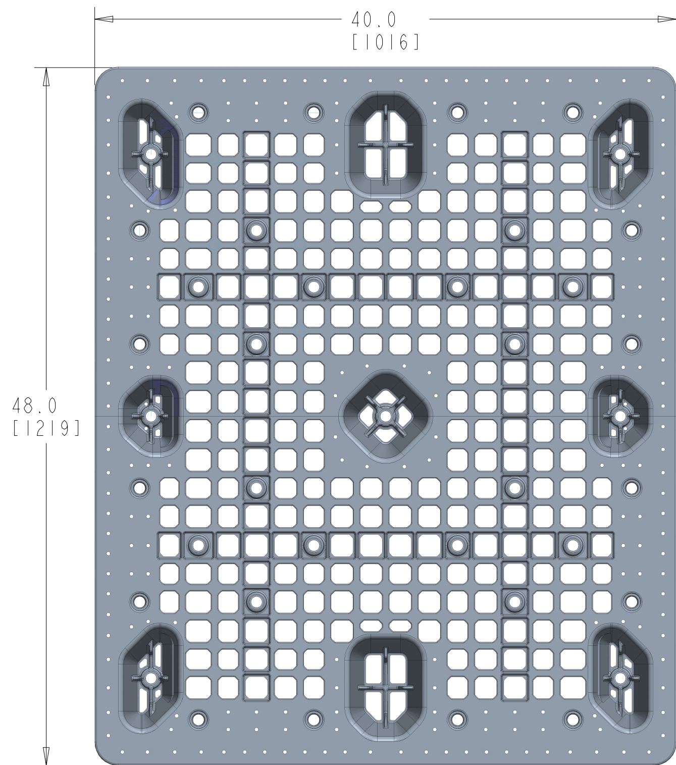
TOP VIEW
