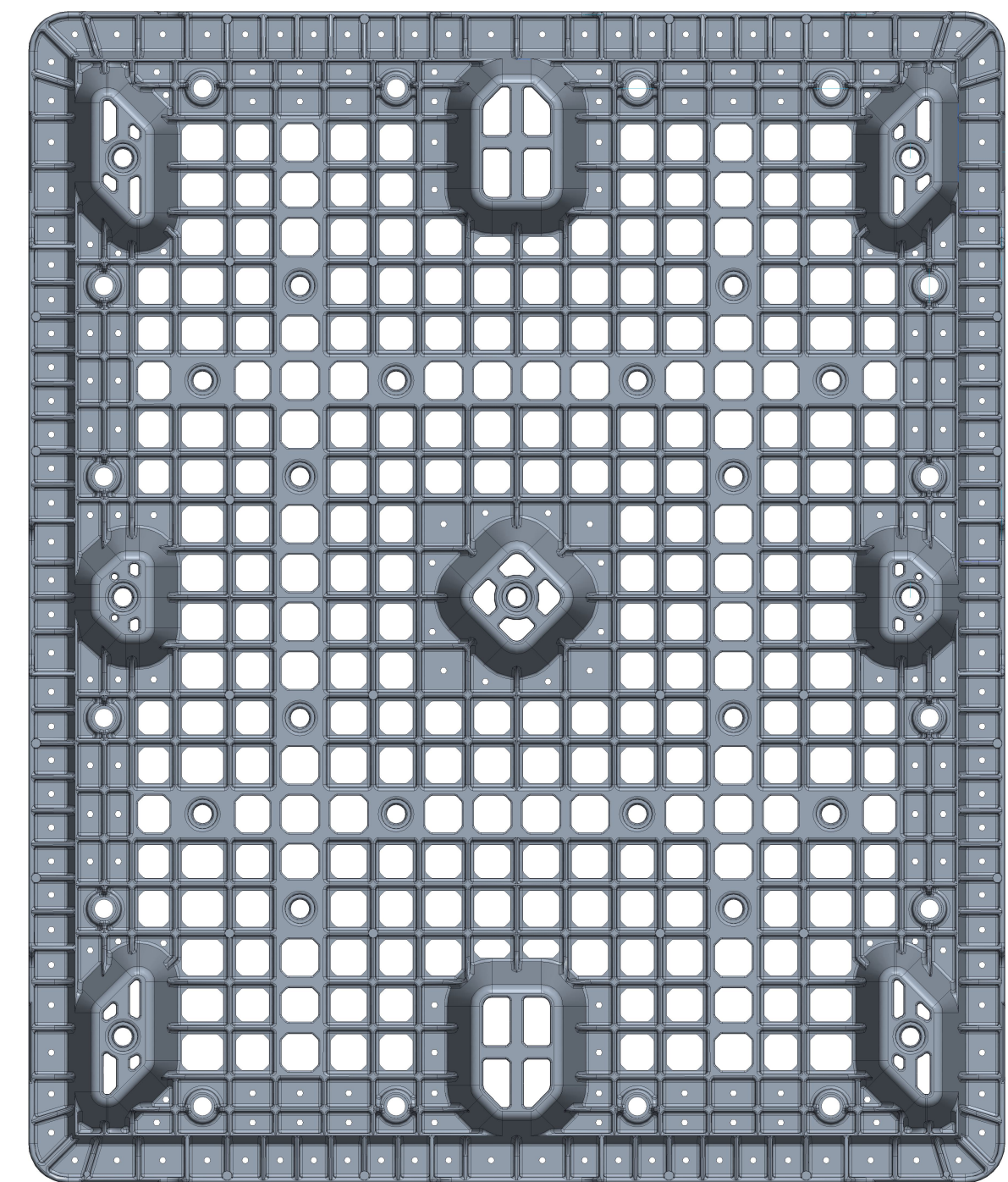
BOTTOM VIEW
