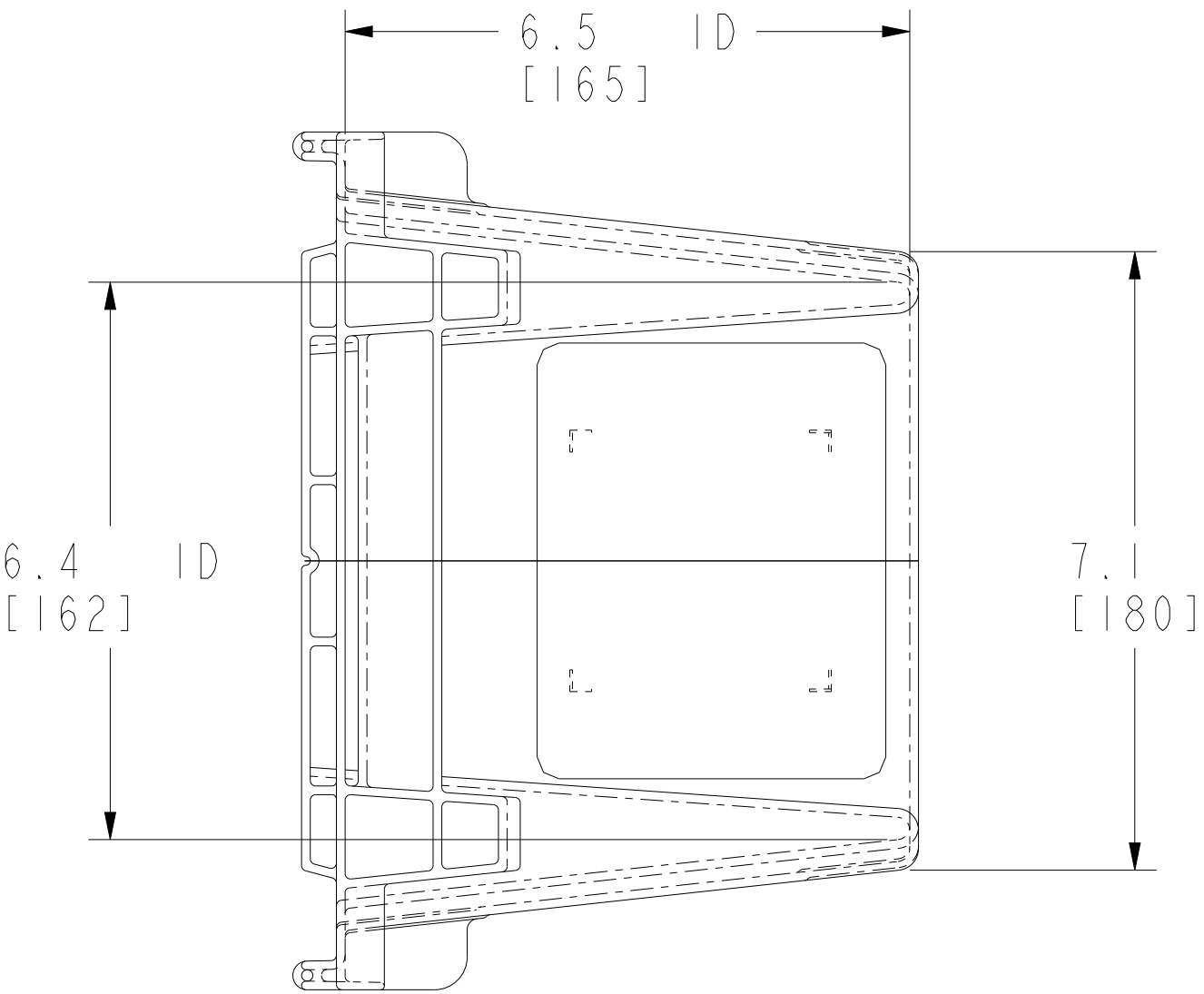
SHORT SIDE
