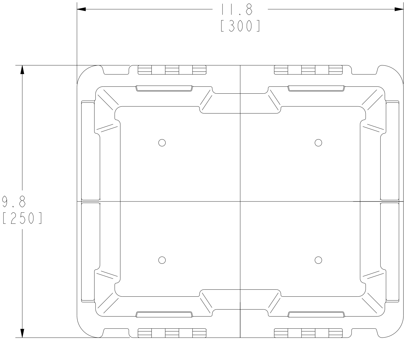
TOP VIEW
