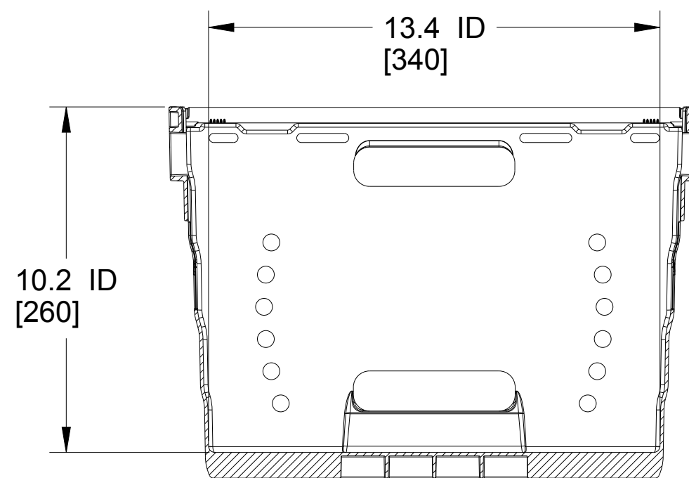
SHORT SIDE
