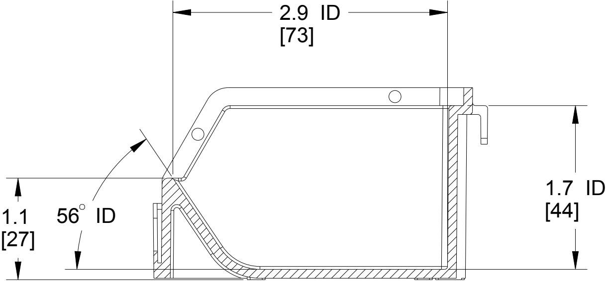
SECTION B-B
