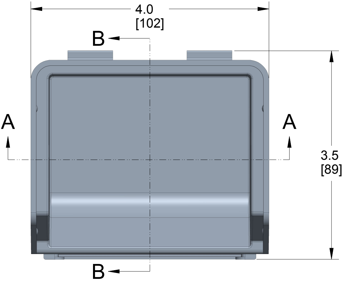
TOP VIEW
