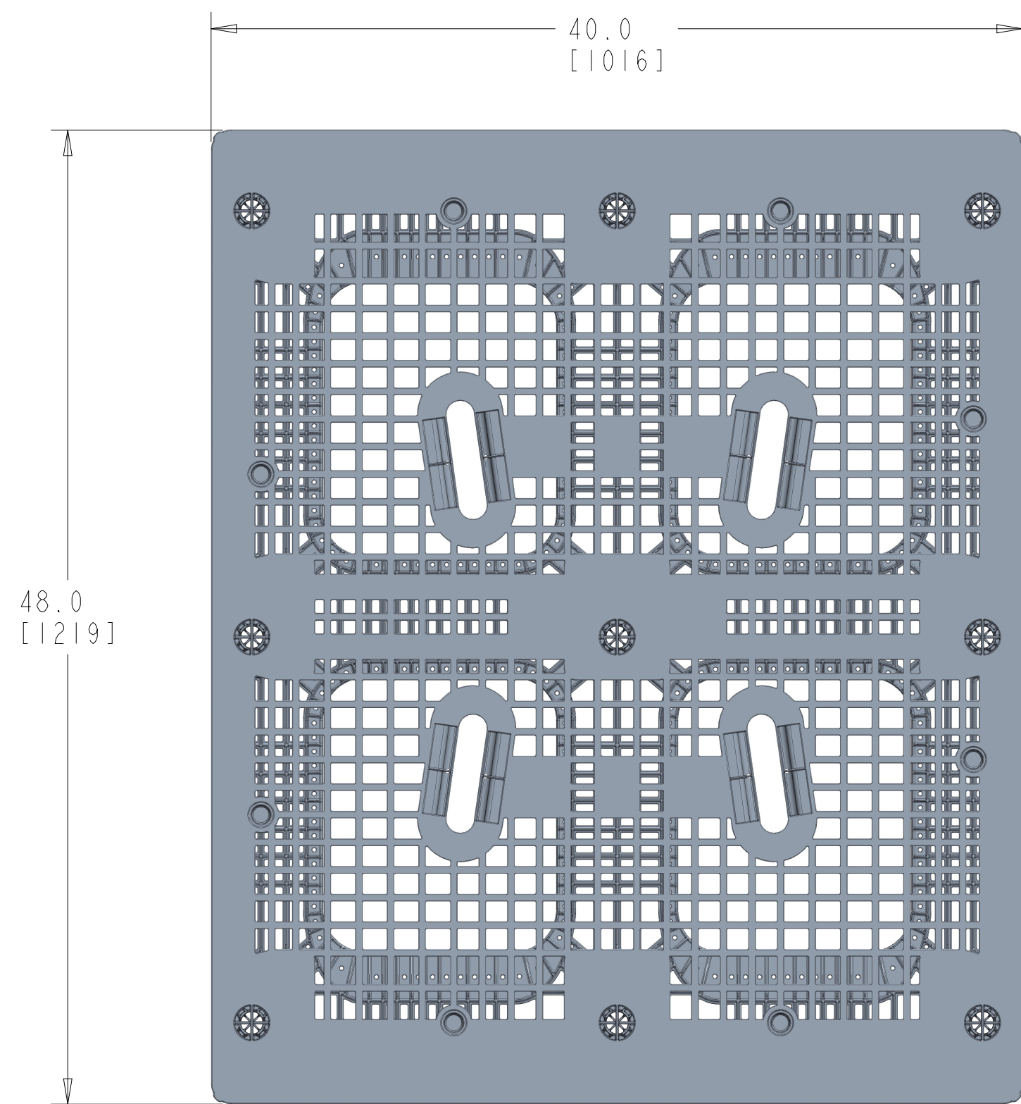
TOP VIEW
