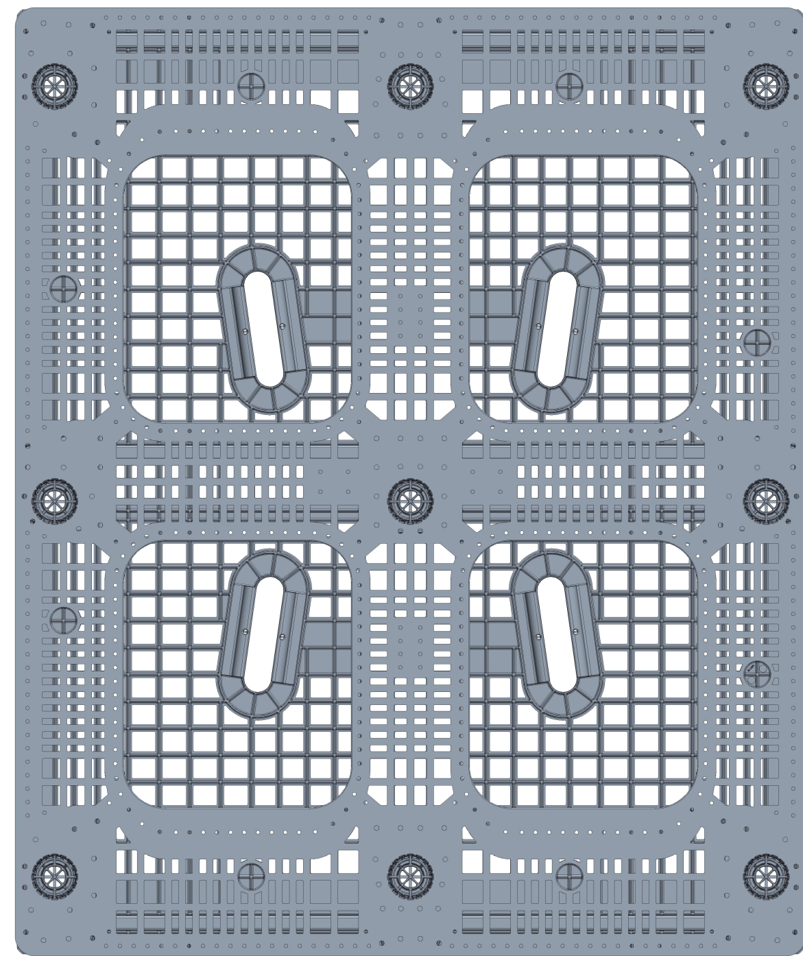
BOTTOM VIEW
