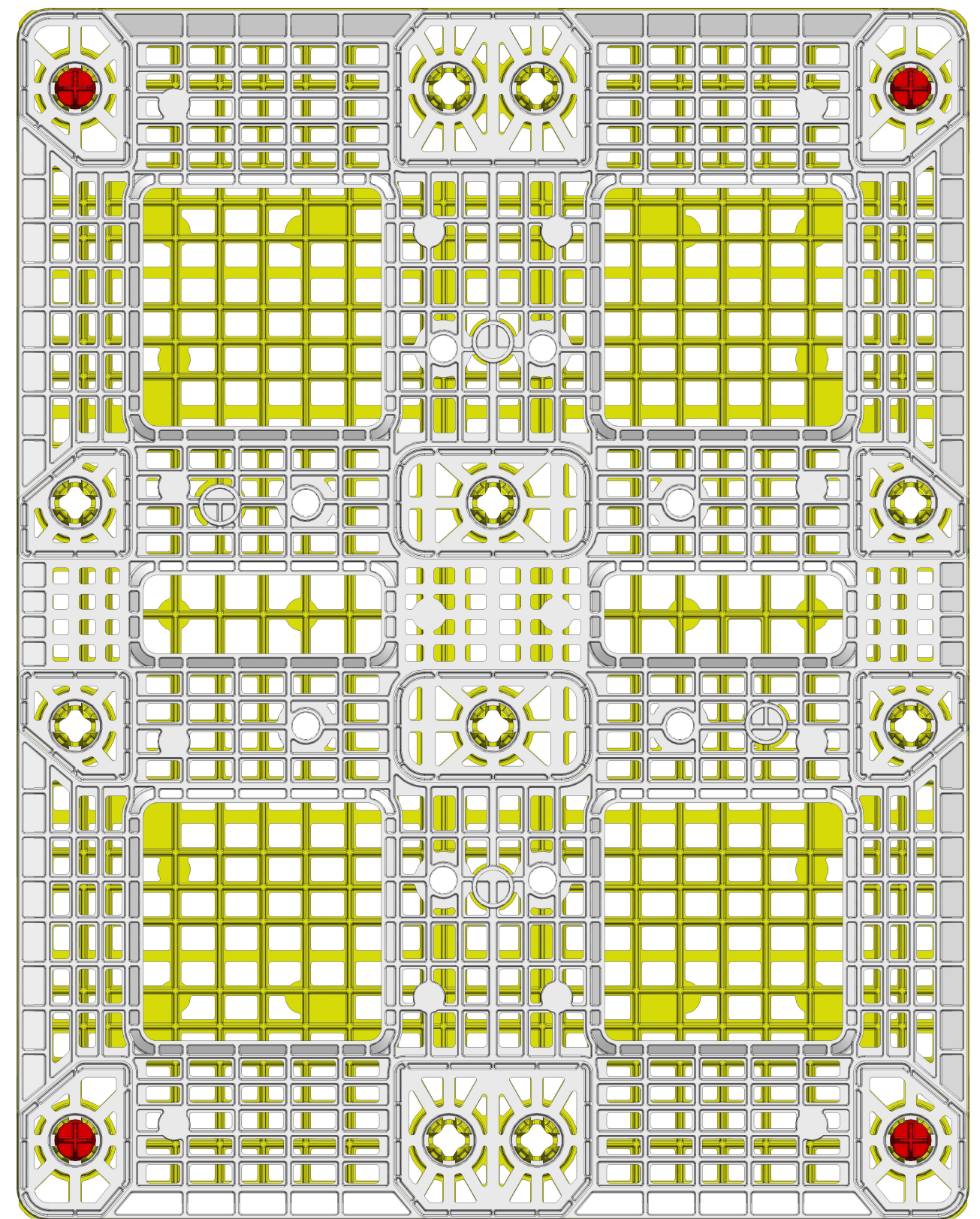
BOTTOM VIEW
