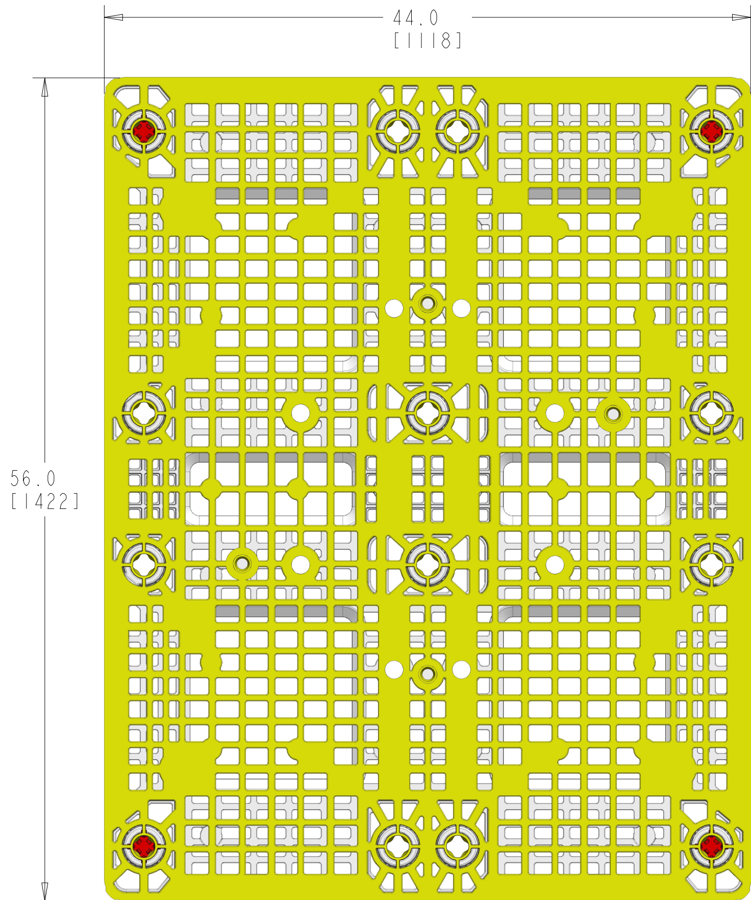
TOP VIEW
