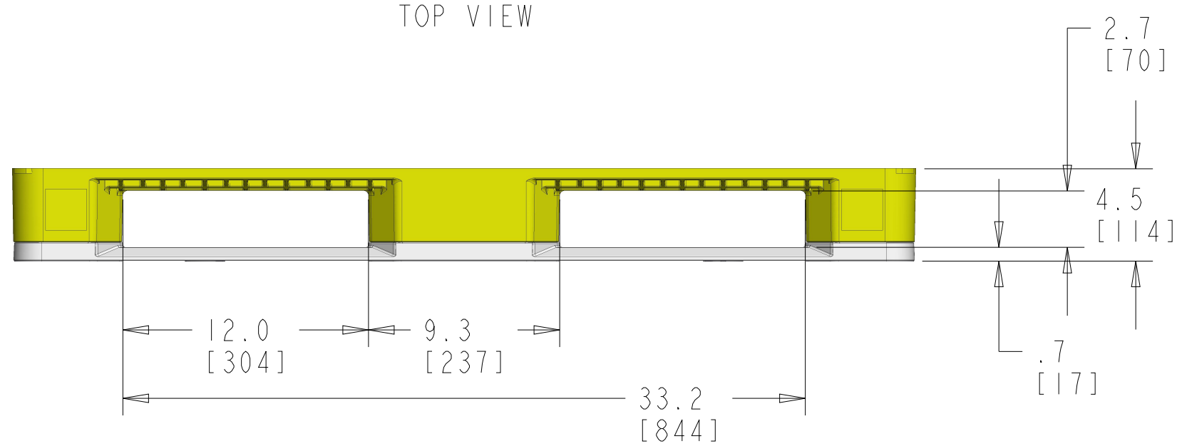
TOP VIEW
