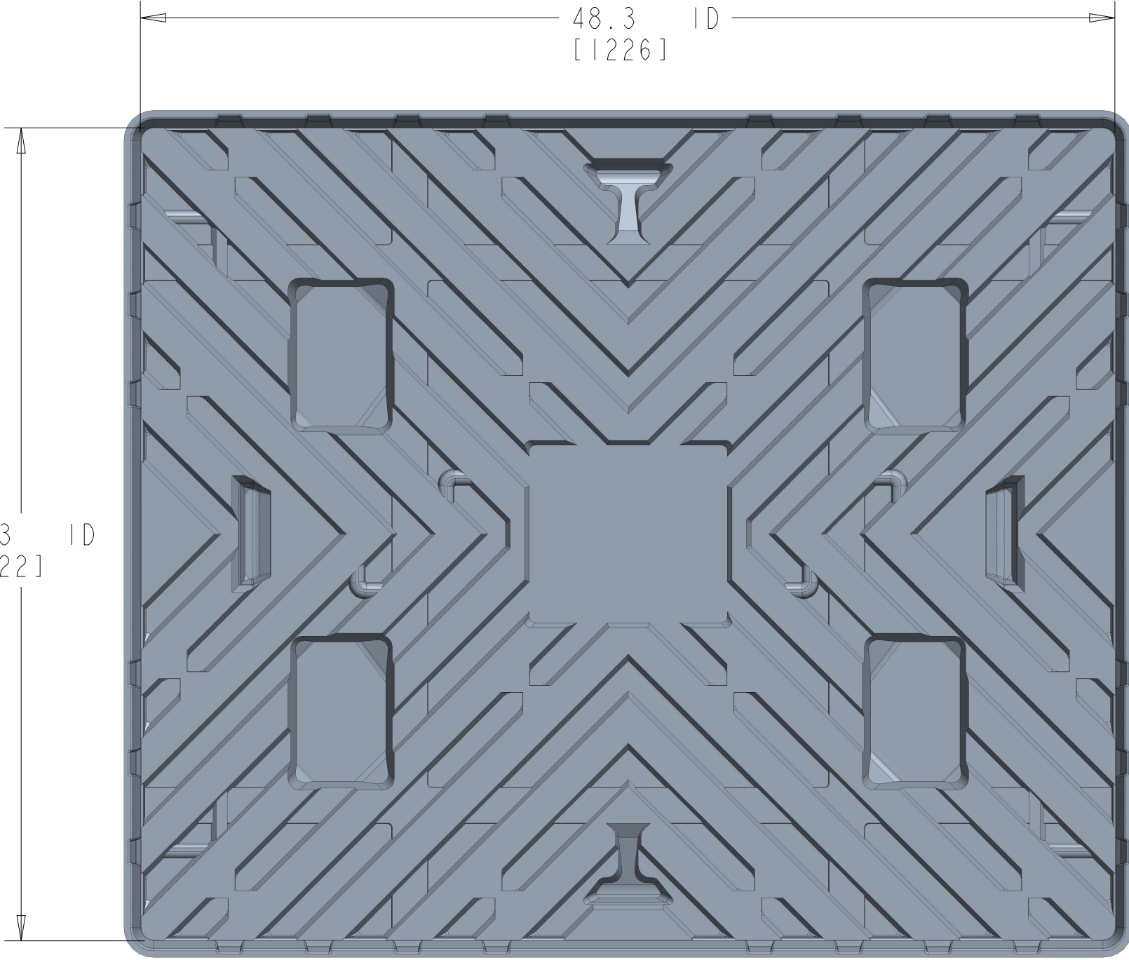
BOTTOM VIEW
