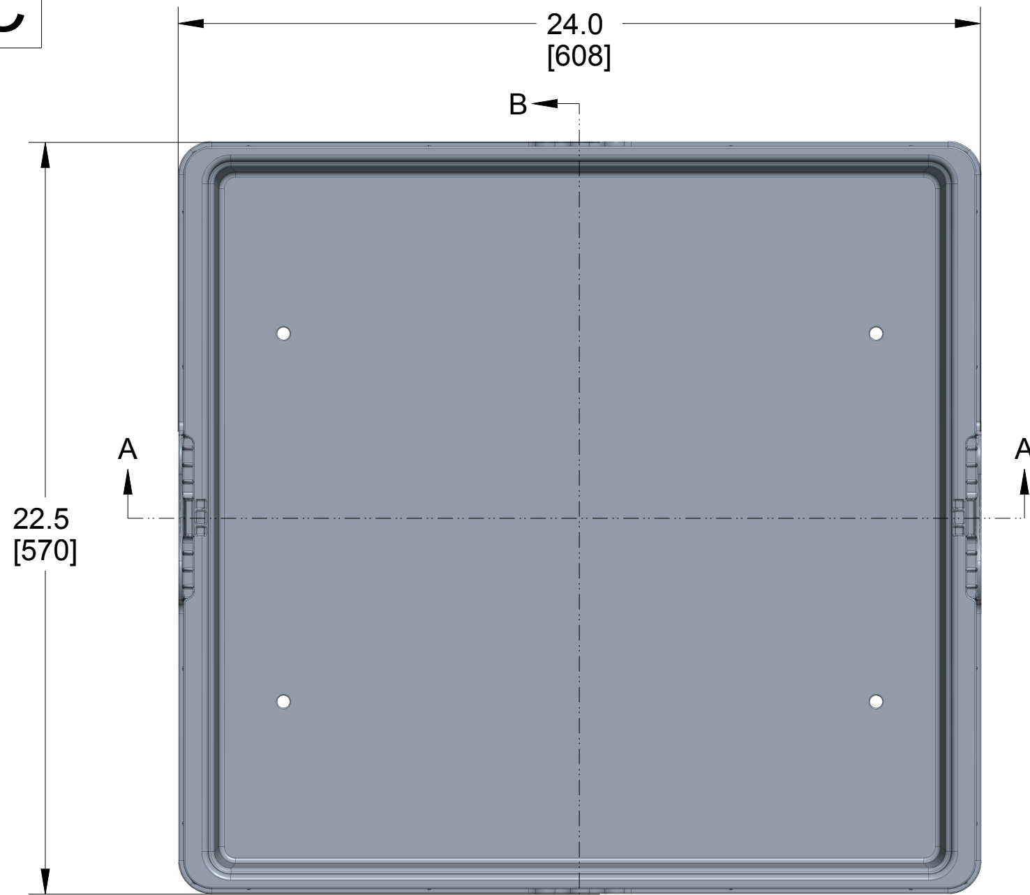
TOP VIEW
