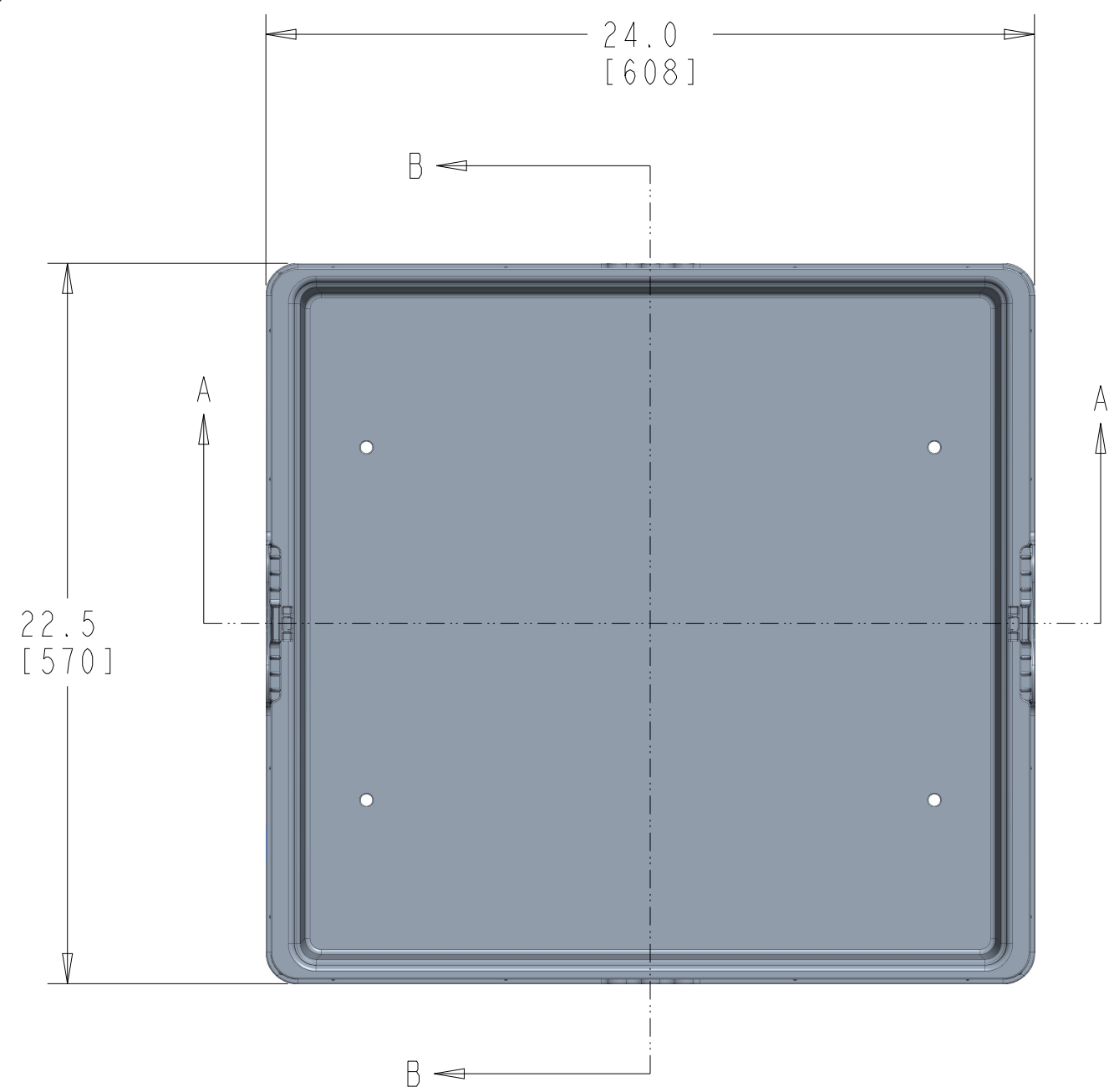
TOP VIEW
