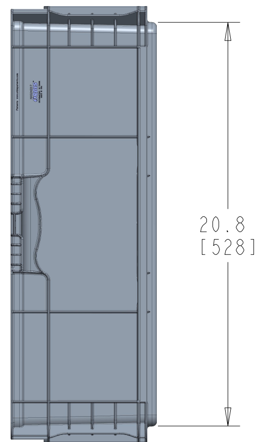
SHORT SIDE
