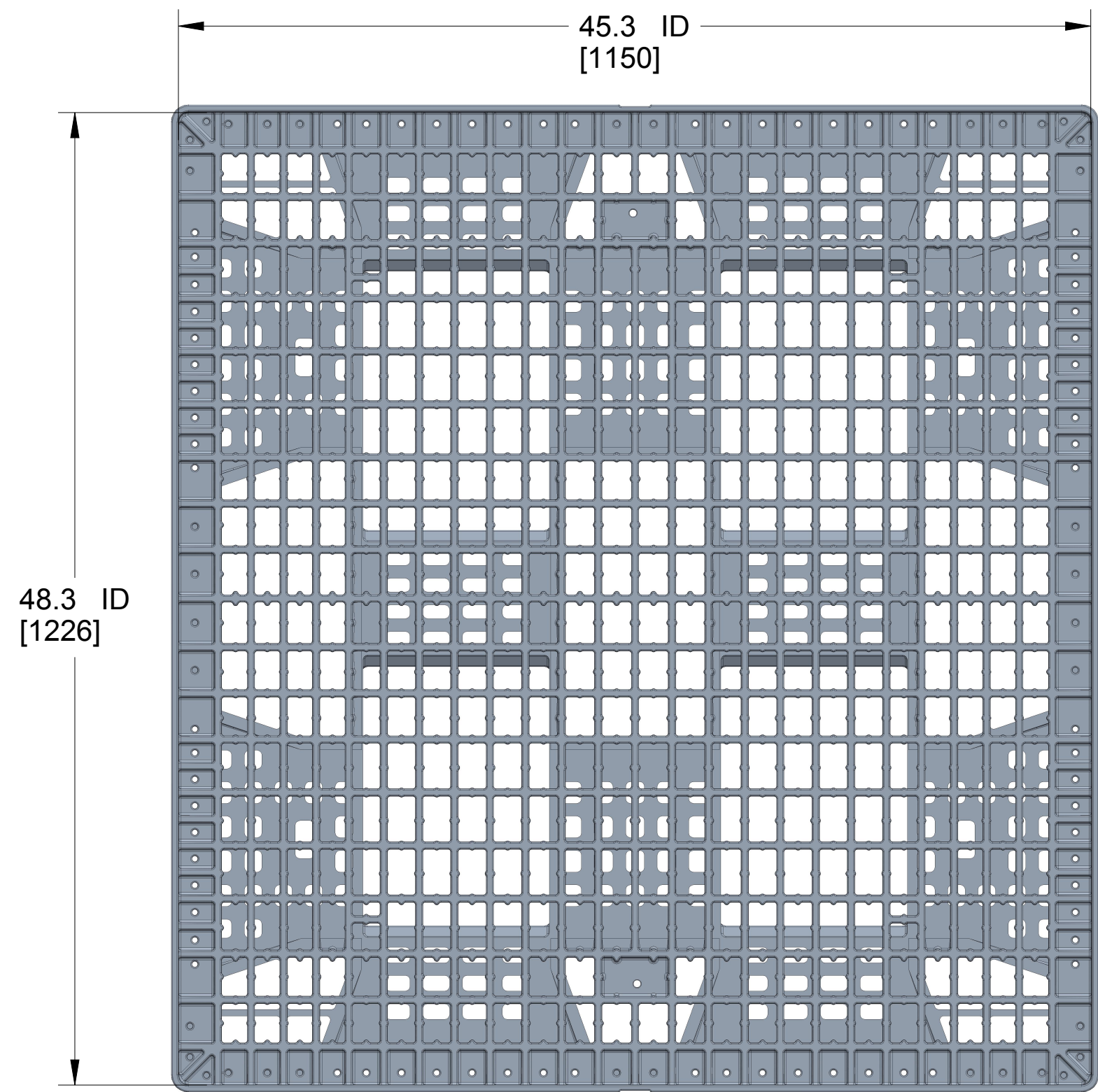
TOP VIEW
